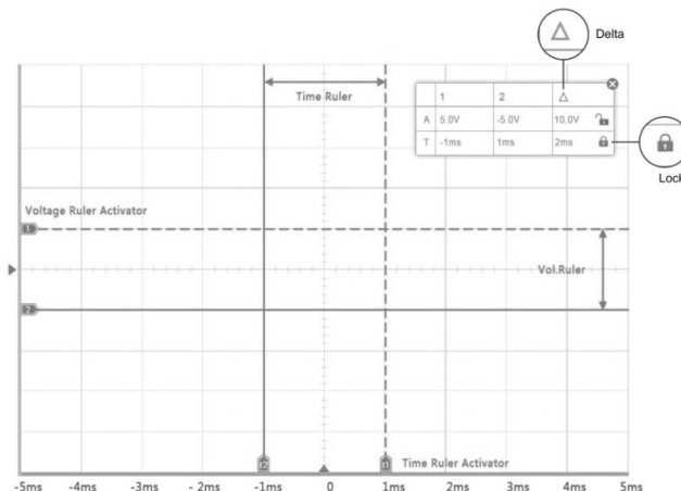
Figure 15-8 Measurement Rulers Display
