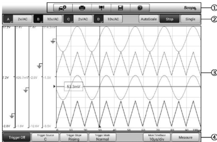
Figure 15-4 Sample MaxiScope Application Screen Layout
